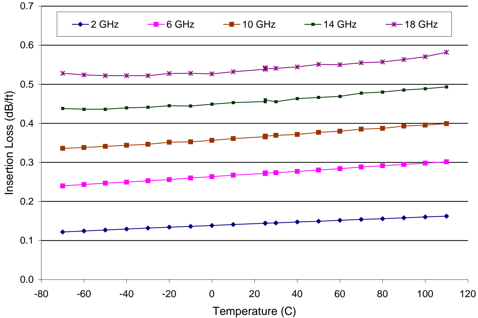
Insertion Loss (dB/ft) vs. Temperature MSSI 0.142" Cable
