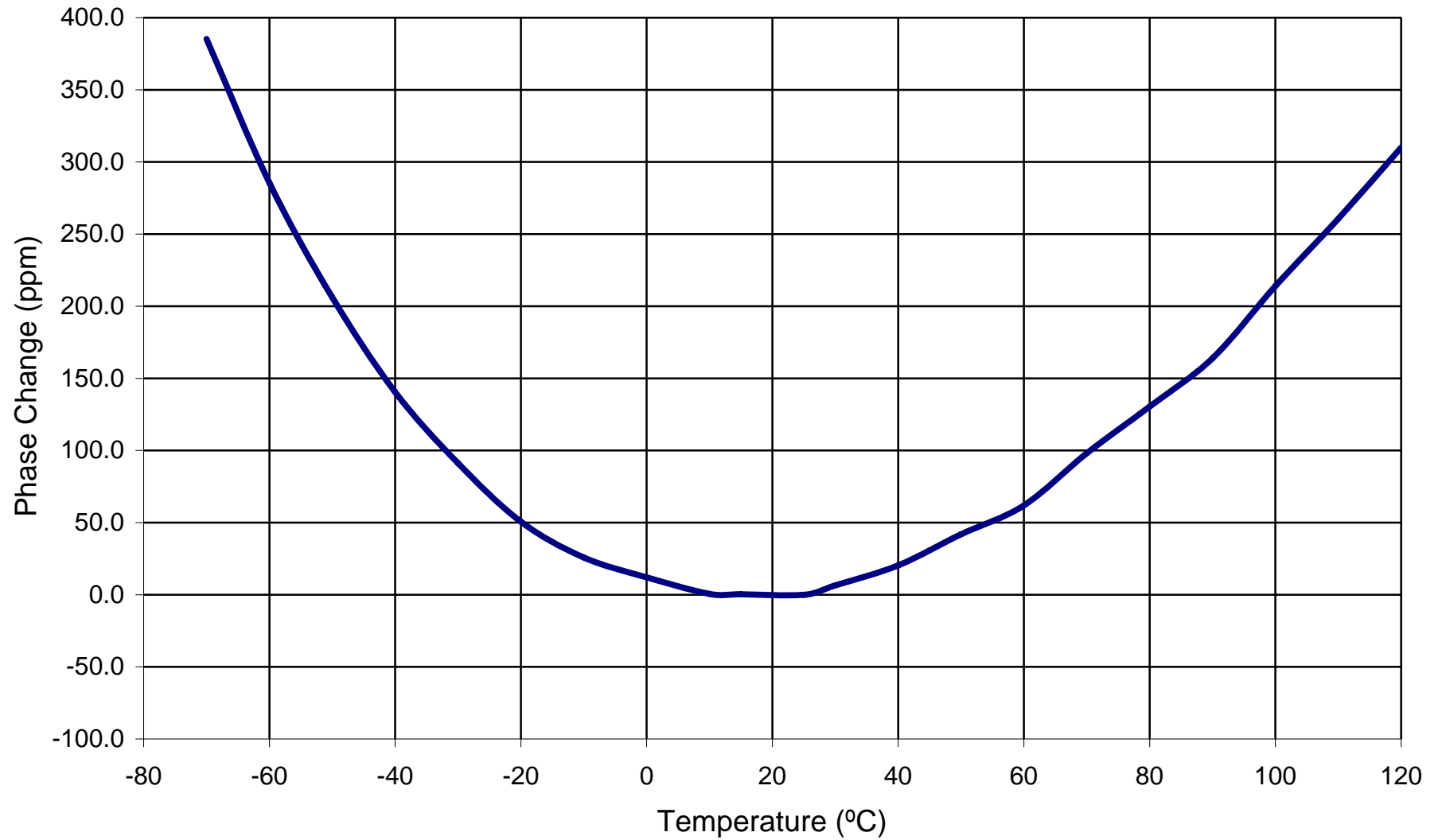
Phase Change From Ambient (ppm) Vs. Temperature (°C) SiO2 Cable
