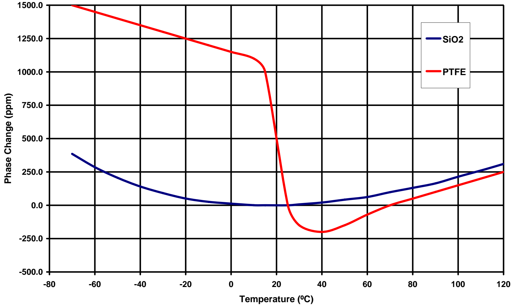
Phase Change From Ambient (ppm) Vs. Temperature (°C) SiO 2 Cable and PTFE Cable
